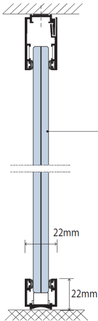
MONO-VETRO SINGLE-GLAZING VITRAGE SIMPLE
