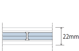
MONO-VETRO SINGLE-GLAZING VITRAGE SIMPLE
