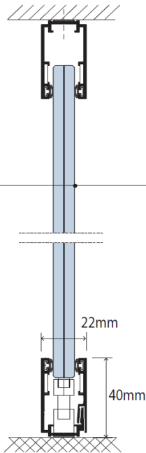
MONO-VETRO SINGLE-GLAZING VITRAGE SIMPLE
