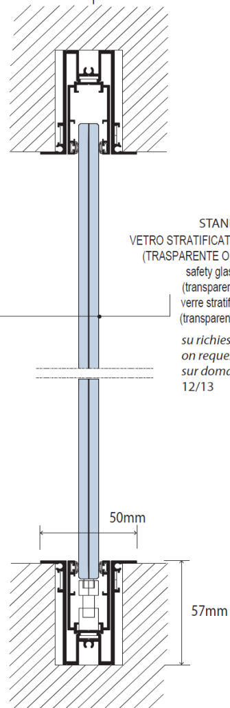
MONO-VETRO INCASSATA BUIL SINGLE-GLAZING VITRAGE SIMPLE ENCASTRE
