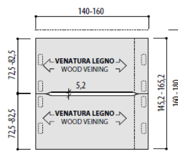
SAGOMATI shaped
